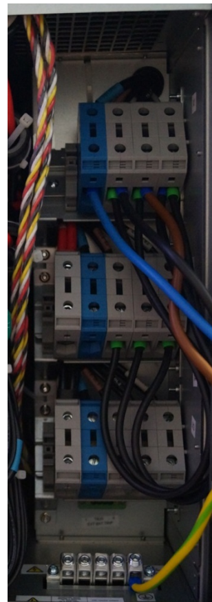
Figure 11. 93PS UPS 30-40 kW power cable terminals
