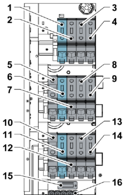
Figure 11. 93PS UPS 30-40 kW power cable terminals
